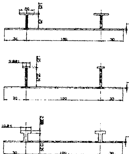
Fig. 19 Shape of stiffener for failure load
