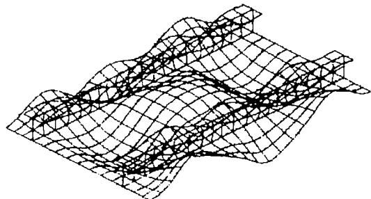
Fig. 3 Deformed shape of post-buckling analysis
