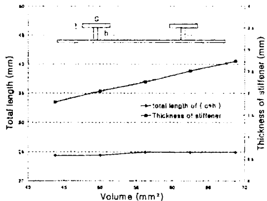
Fig. 16 Variation of thickness and total length for the increase of volume of stiffener
