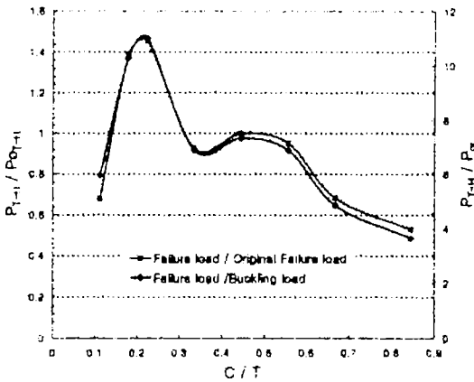
Fig. 10 Variation of nondimensional failure load for aspect ratio
