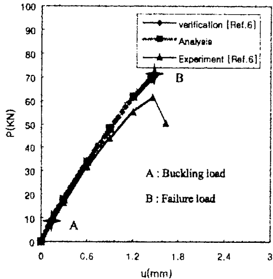
Fig. 4 Comparison of experiment results and analysis results of load-shortening displacement curve
